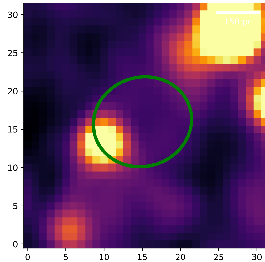
IRAC 8 micron - Classification: Clumpy
