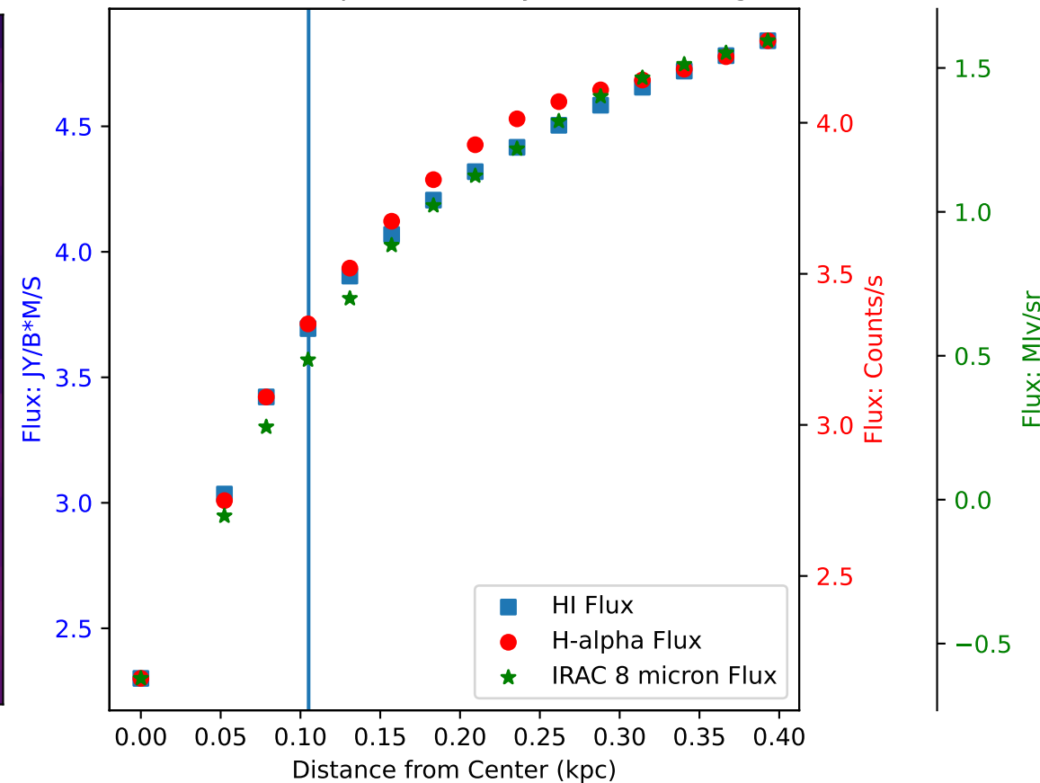
Flux of HI vs. H-alpha in Galaxy: DDO 53 - Region 2
