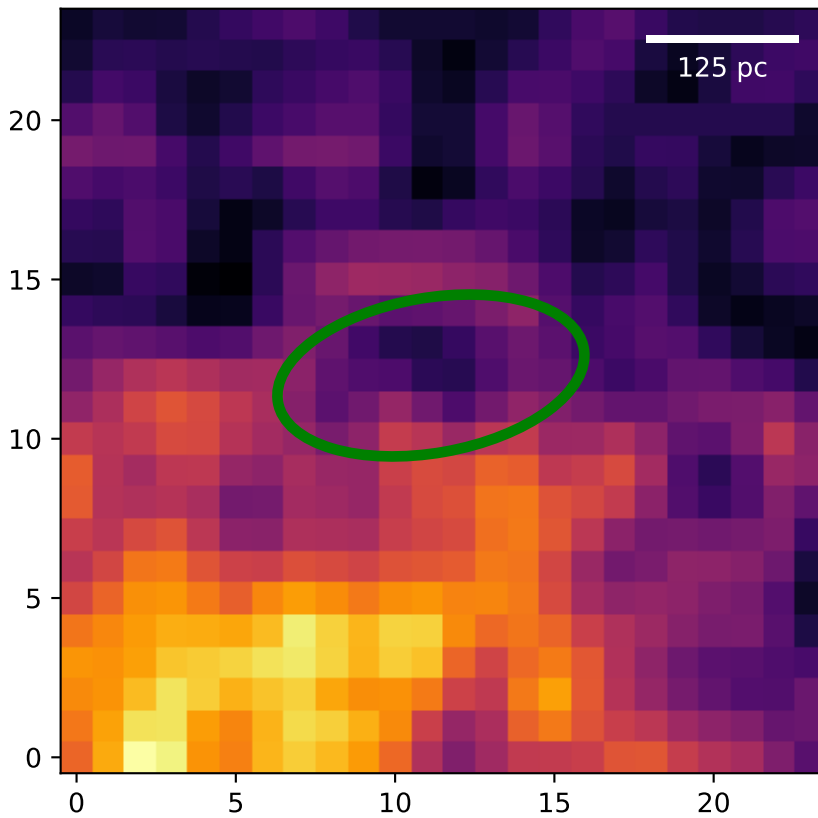
Region: 5 HI - Type 3
