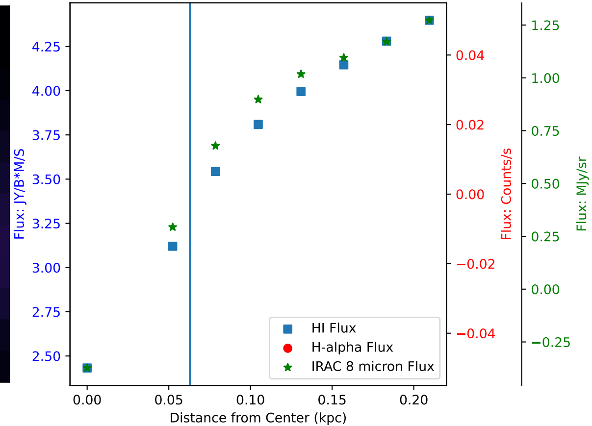
Flux of HI vs. H-alpha in Galaxy: DDO 53 - Region 3
