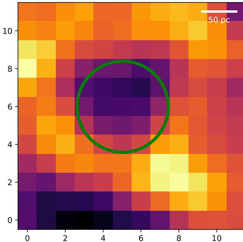
Region: 3 HI - Type 3
