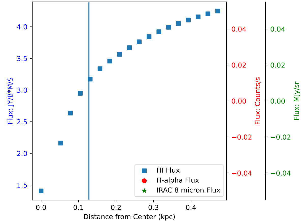
Flux of HI vs. H-alpha in Galaxy: DDO 53 - Region 5
