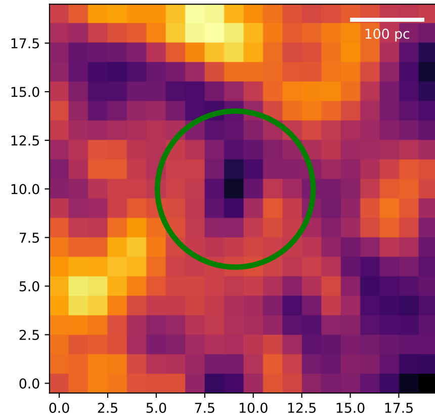
Region: 2 HI - Type 3
