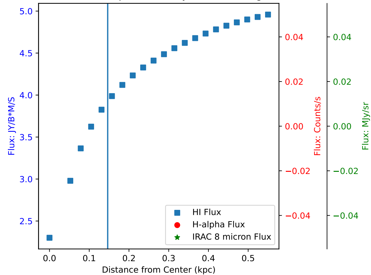
Flux of HI vs. H-alpha in Galaxy: DDO 53 - Region 7
