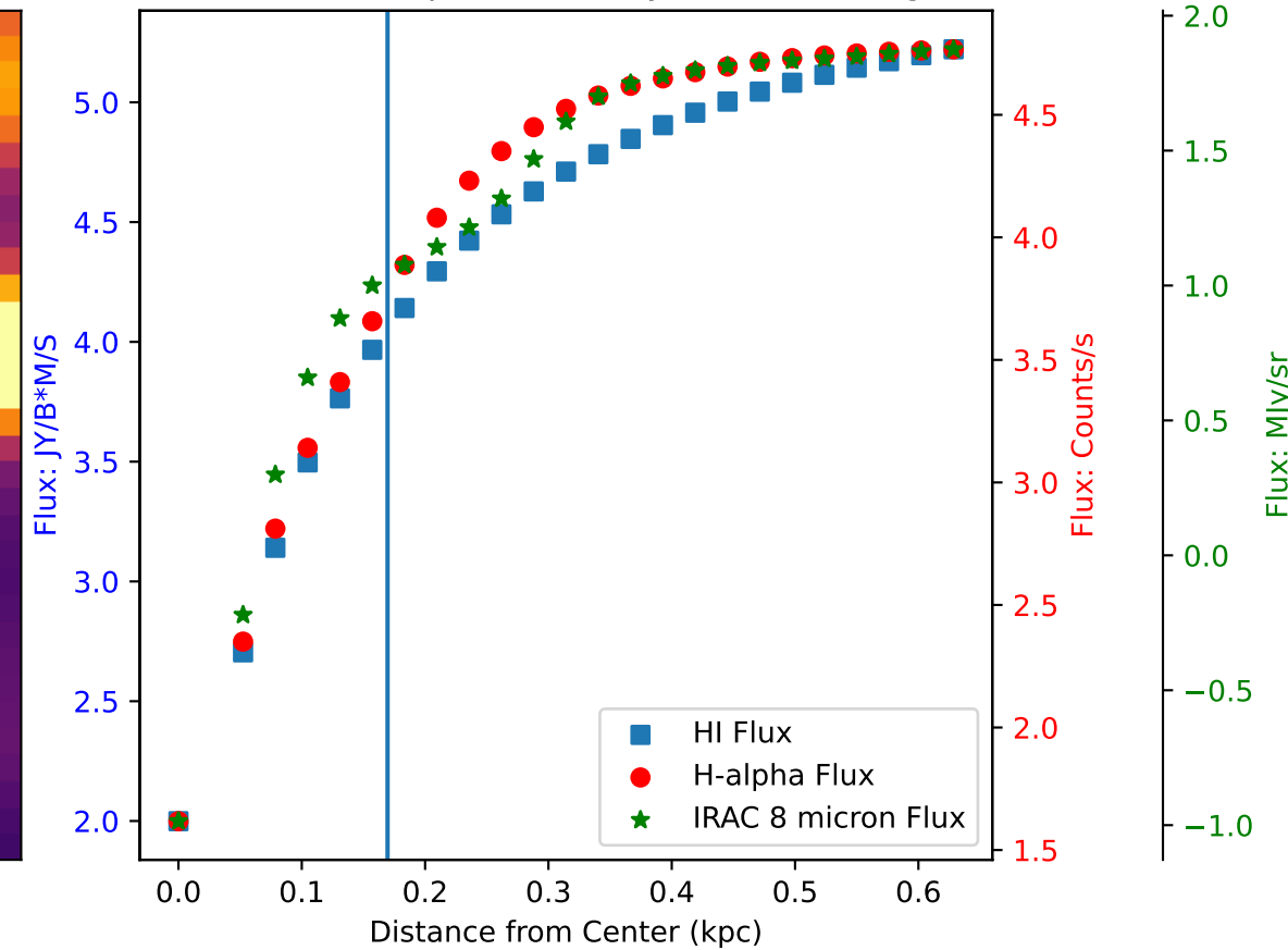
Flux of HI vs. H-alpha in Galaxy: DDO 53 - Region 6
