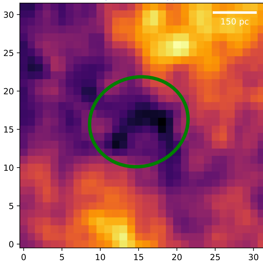
Region: 6 HI - Type 1
