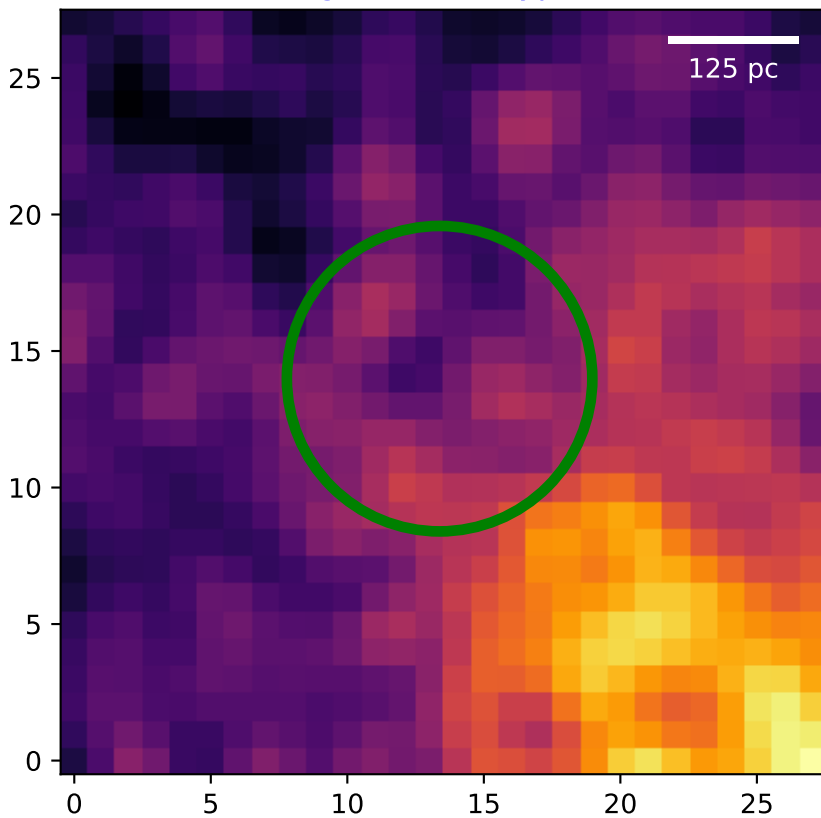
Region: 7 HI - Type 3
