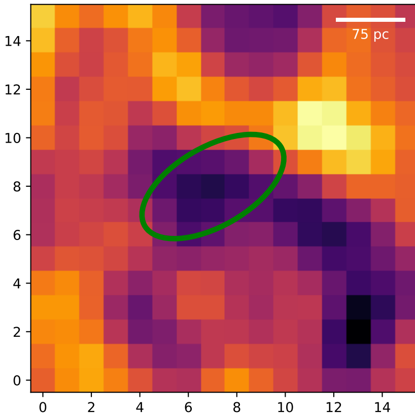
Region: 4 HI - Type 3
