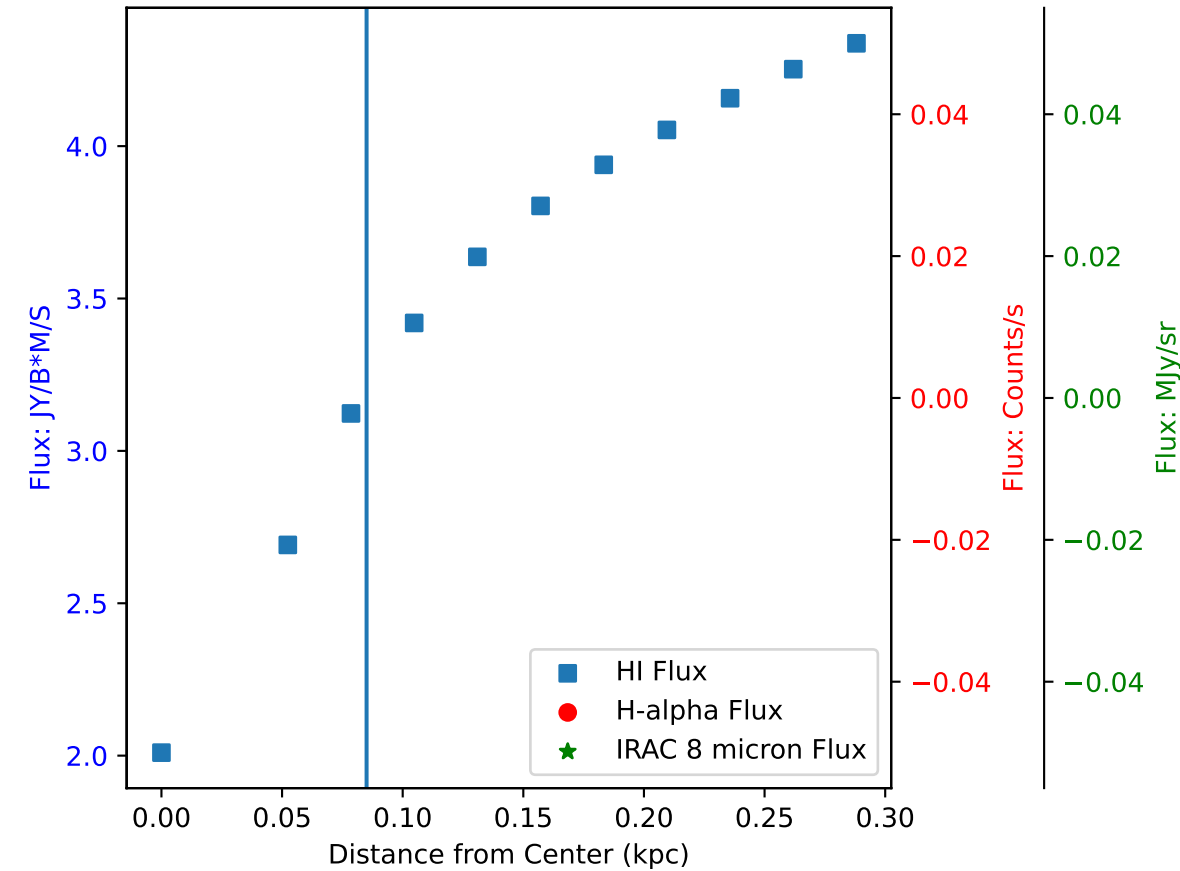
Flux of HI vs. H-alpha in Galaxy: DDO 53 - Region 4
