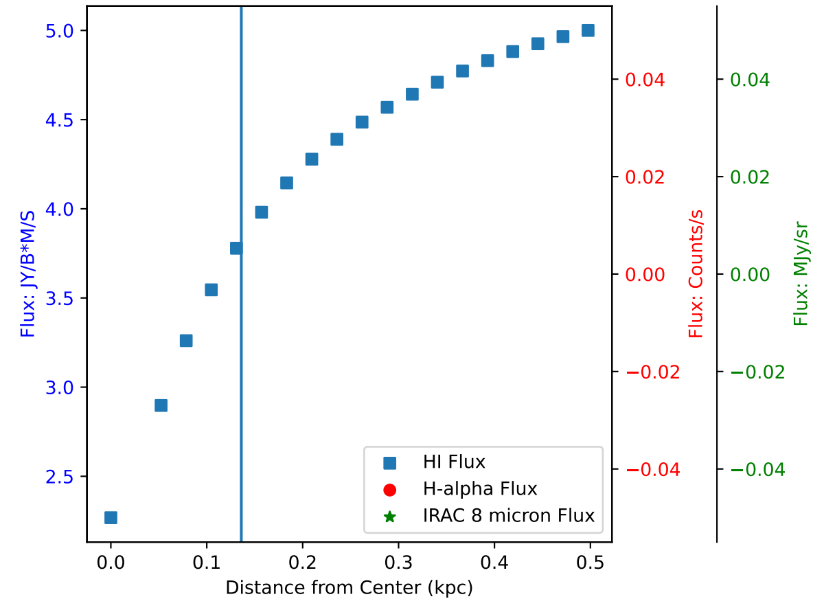
Flux of HI vs. H-alpha in Galaxy: DDO 53 - Region 1
